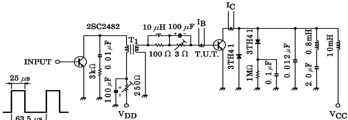
Fig.1 SWITCHING TIME TEST CIRCUIT
